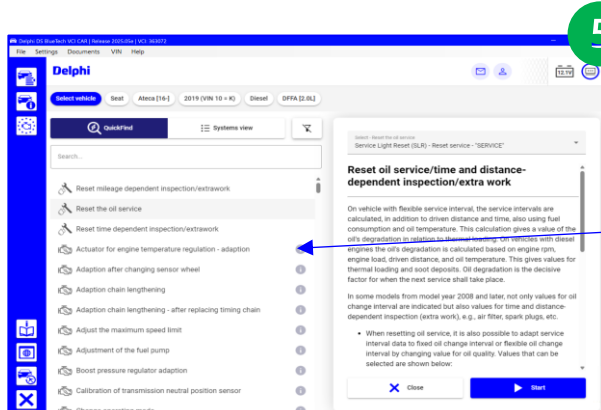
QuickFind filter can be removed, and the details of the functions can be viewed.
