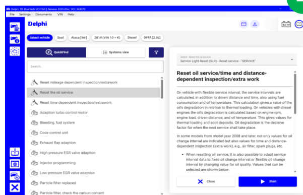
QuickFind filtered with function details
