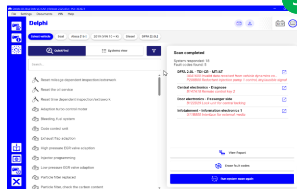
QuickFind filtered after the scan
